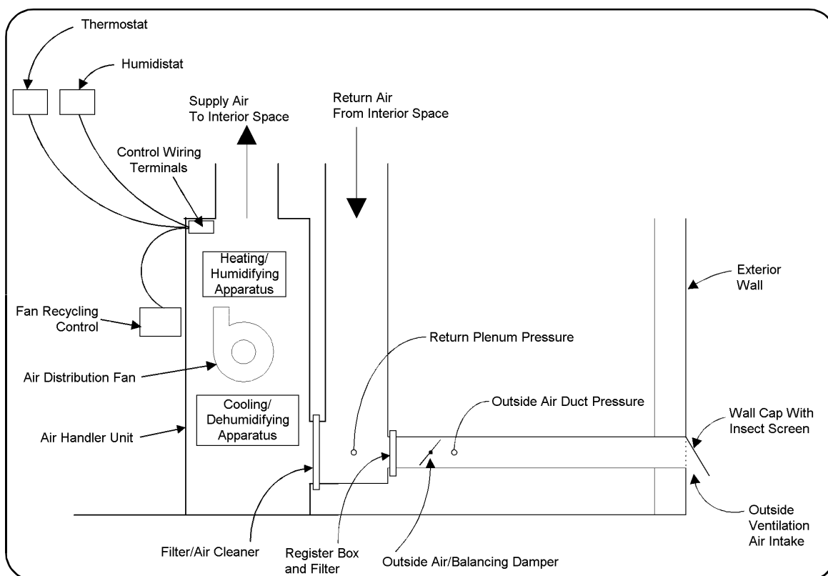
Figure 1 Diagram for one configuration of a central-fan-integrated supply ventilation system using an outside air duct to the return side of a central air distribution fan
